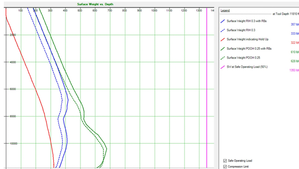
A Cerberus™ surface weight plot showing results for the same tool string with and without Roller Bogies®
